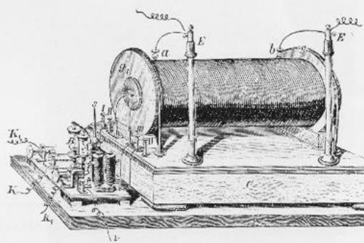
Ruhmkorff induction coil. 5
