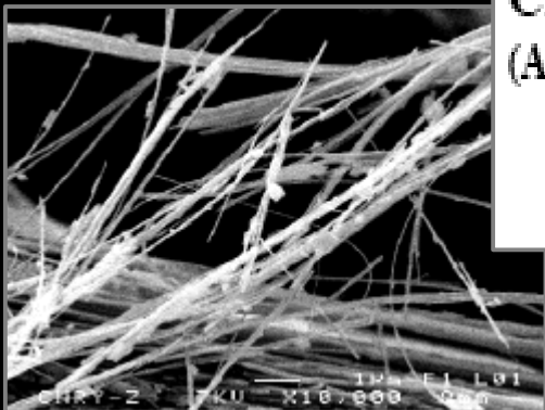
Chrysotile
